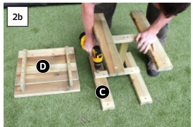
Attach bracing assembly to Legs C (200mm from base of Legs) using 8no Screws (Figs.2a & 2b).
