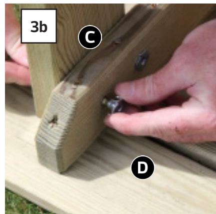
Position leg assembly onto Table Top D (Fig.3a). Align bolt holes and insert 2no Hex Bolts and 'T' Nuts per Leg (Fig.3b). Fully tighten all bolts (Fig.3c).
