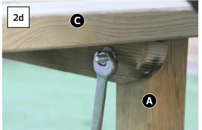
Position Table Top C onto Side Panels A (Fig.2a), align bolt holes and fix in position using 4no Bolts, Washers and Nuts – 2no per side (Figs.2b, 2c & 2d).
