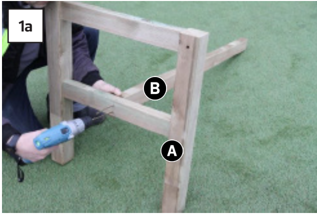
Attach Side Panels A to Bracing B as shown in Figs.1a & 1b using 4no Screws (2no per side)
