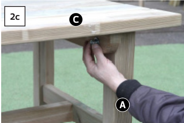
Position Table Top C onto Side Panels A (Fig.2a), align bolt holes and fix in position using 4no Bolts, Washers and Nuts – 2no per side (Figs.2b, 2c & 2d).
