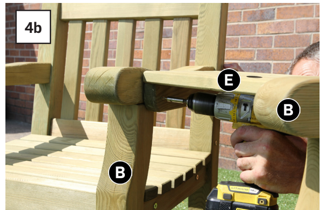
Position Upper Shelf Assembly E between seats and attach using 4x 60mm Screws - 2 per side (Figs.4a & 4b).
