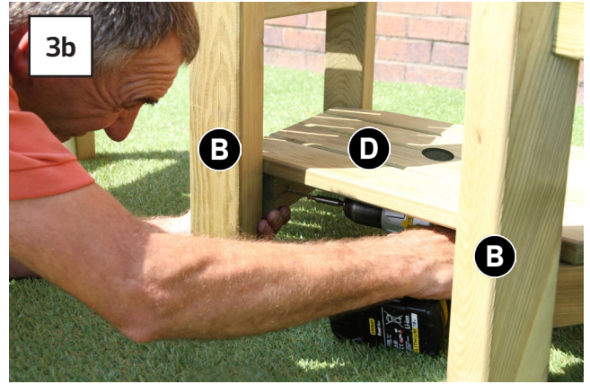
Locate Lower Shelf Assembly D between seats and attach using 4x 60mm Screws - 2 per side (Figs.3a & 3b).
