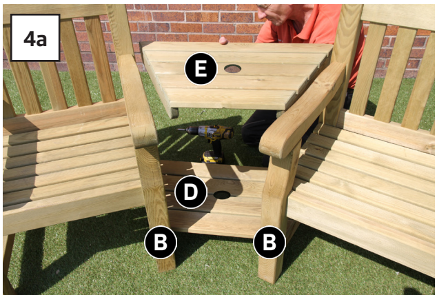
Position Upper Shelf Assembly E between seats and attach using 4x 60mm Screws - 2 per side (Figs.4a & 4b).
