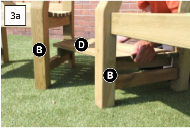
Locate Lower Shelf Assembly D between seats and attach using 4x 60mm Screws - 2 per side (Figs.3a & 3b).
